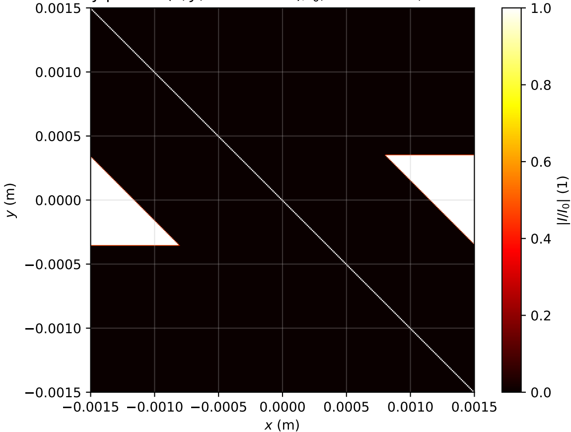
Intensity profile I(x, y, z = 0.000\text{m})/I_0 , \text{Pin}=8.0\text{Pcr} , artificial time
